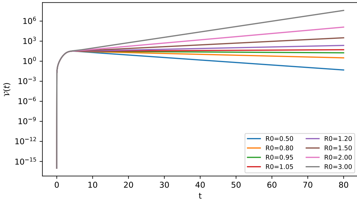
Test F: R_0 threshold scan ( \mu = 0, \delta = 0.1 )
